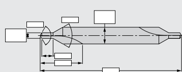
CENTER DRILL
